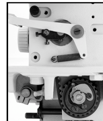
Built-in safety clutch system prevents hook damage
